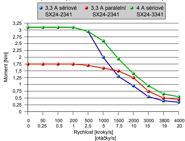
Momentová charakteristika motoru SX24-2341 s CD30x, CD30M (48 VDC), SX24-3341 s CD40x, CD40M (48 VDC)
